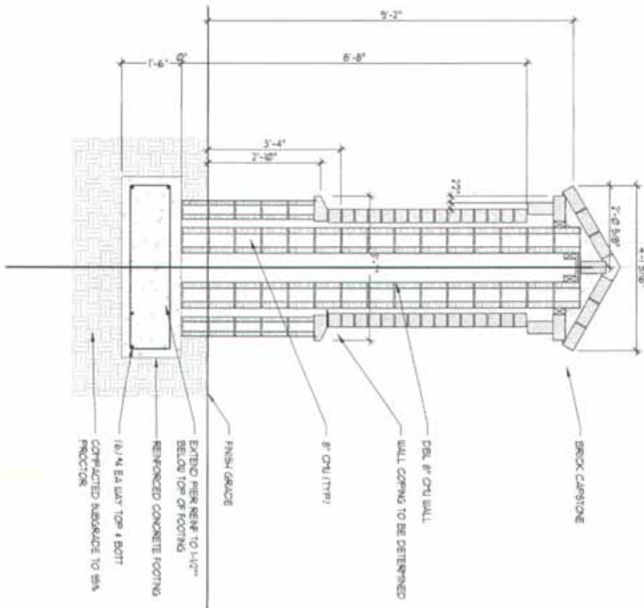
2 SECT THRU PILASTER AL-02 SCALE 1/4" = 1'-0"
